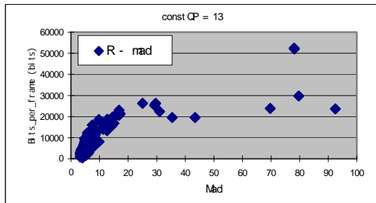
Fig. 1: R - mad data for the movie sequence ‘‘Hangingup’’ with constant QP. ‘‘Hangingup’’: 320x224, 300 frames, lots of scene change and high motion
